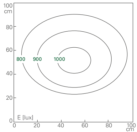
ECO VERSION SYSTEMLED ECO 28W / 898mm opalweiß / milky
